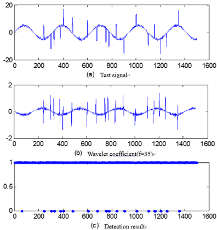
Figure 1: Electrode regulation system signal and test result
