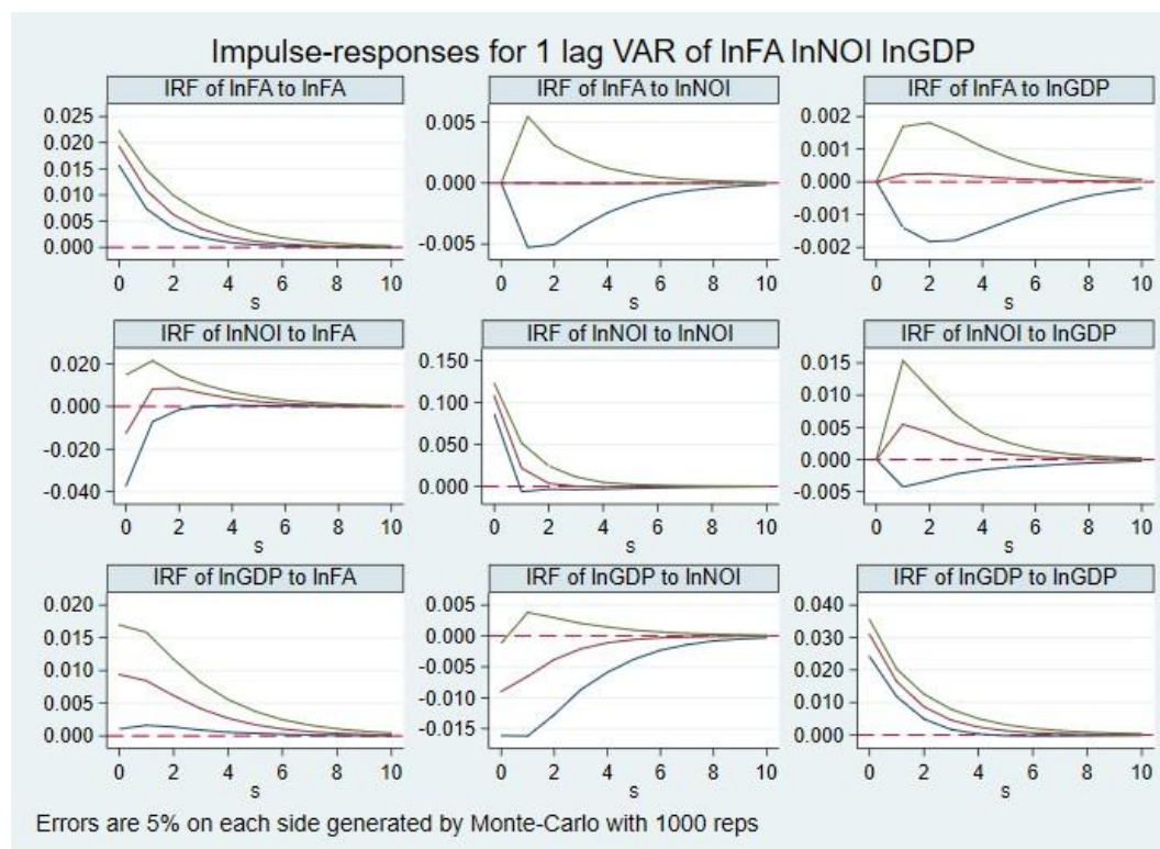
Figure 2: PVAR model impulse response function
